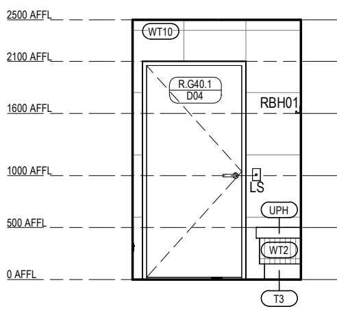
STAFF SHOWER ELEVATION 3 Scale 1: 50
