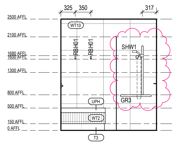
STAFF SHOWER ELEVATION 2 Scale 1: 50
