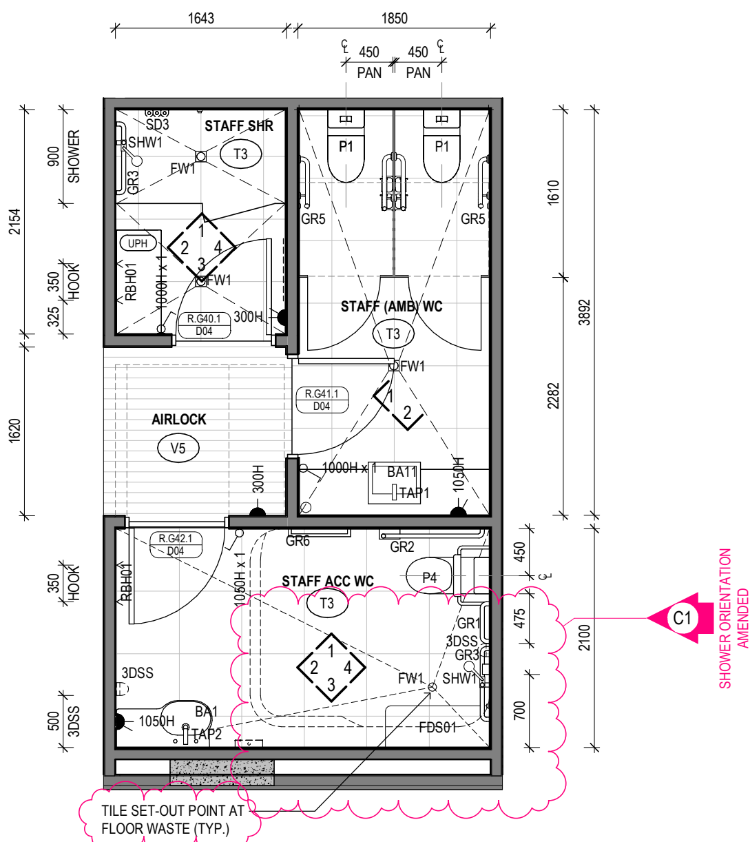
1 VILLAGE ADMIN - STAFF AMENITIES Scale 1: 50
