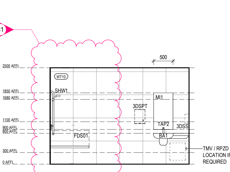
STAFF ACCESSIBLE WC ELEVATION 3 Scale 1: 50
