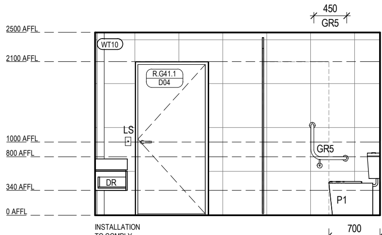
STAFF AMBULANT WC ELEVATION 1 Scale 1: 50
