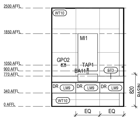
STAFF AMBULANT WC ELEVATION 2 Scale 1: 50
