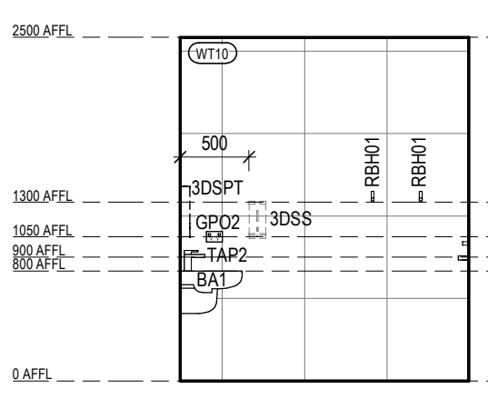
STAFF ACCESSIBLE WC ELEVATION 2 Scale 1: 50
