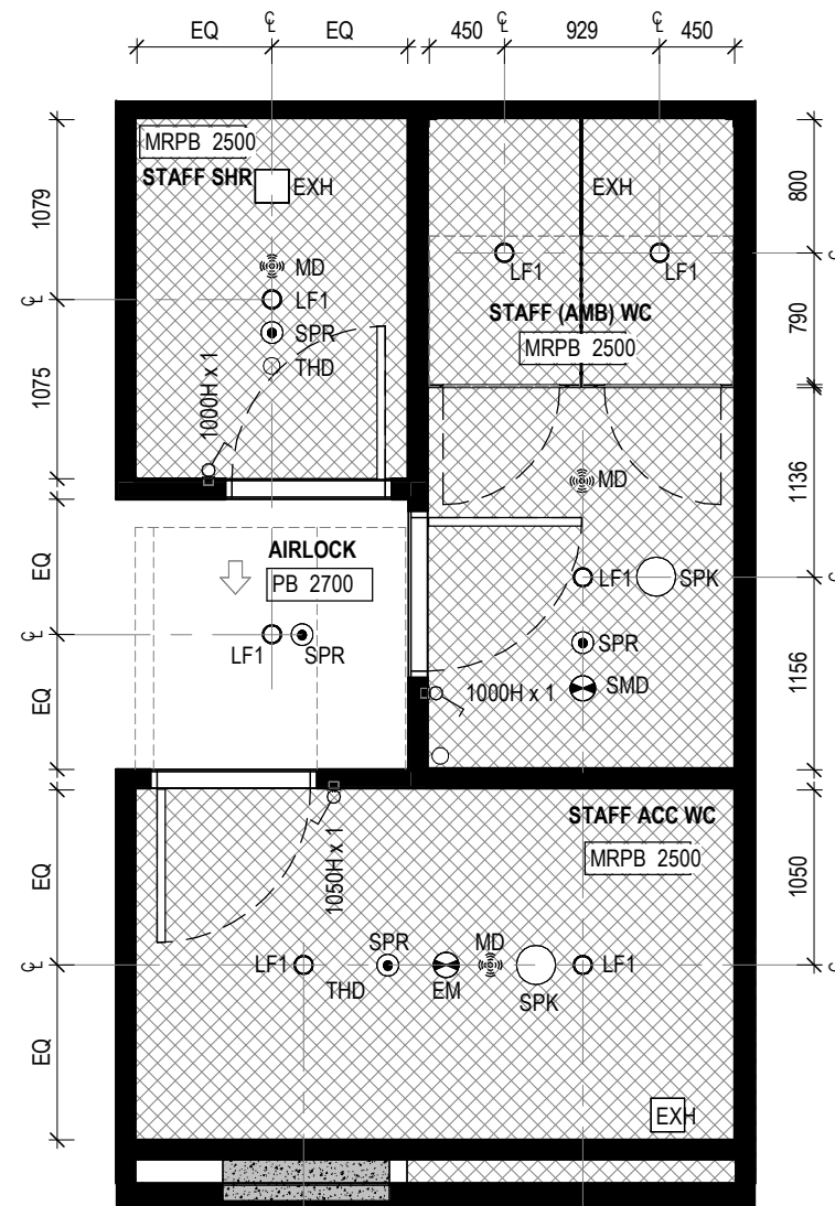
2 RCP - VILLAGE ADMIN - STAFF AMENITIES Scale 1: 50
