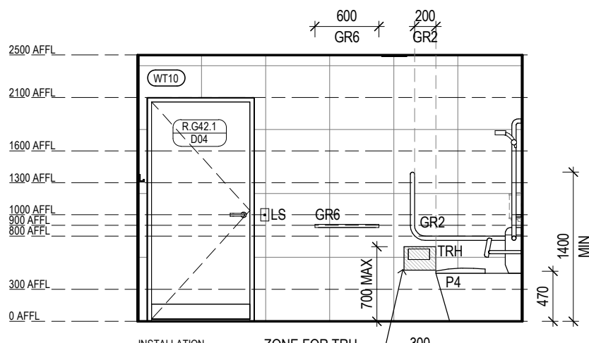
STAFF ACCESSIBLE WC ELEVATION 1 Scale 1: 50
