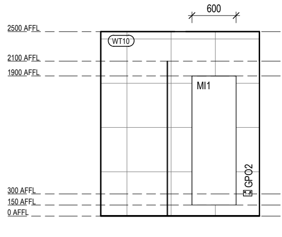
STAFF SHOWER ELEVATION 4 Scale 1: 50
