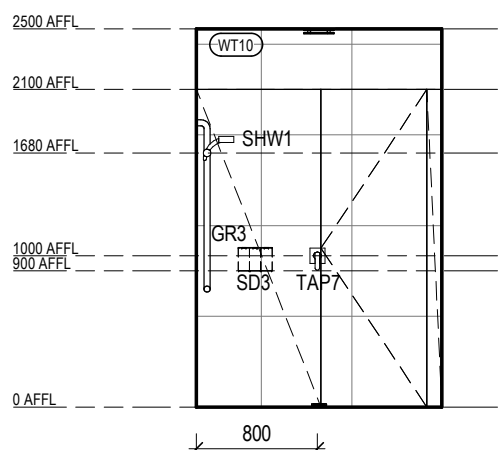
STAFF SHOWER ELEVATION 1 Scale 1: 50
