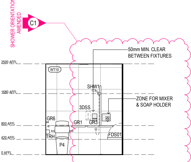
STAFF ACCESSIBLE WC ELEVATION 4 Scale 1: 50
